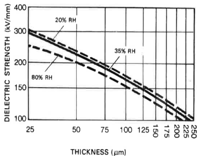
Figure 3 Dielectric Strength at Various Levels of Humidity
